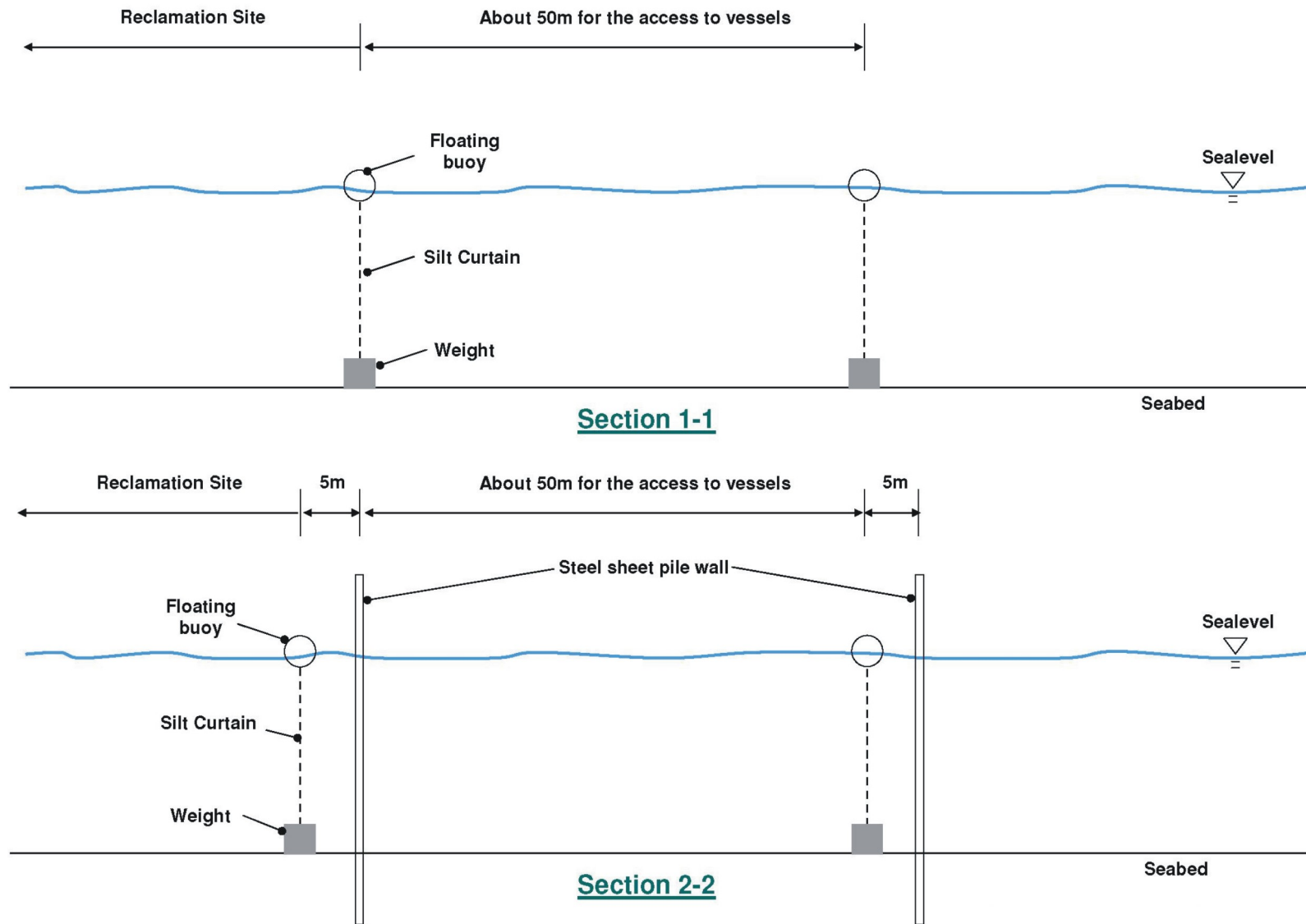
Figure 6 - Details of Silt Curtains and Steel Sheet Pile Wall
